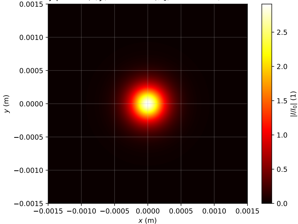
Intensity profile I(x, y, z = 3.423m)/I_0 , Pin=1.0Pcr, artificial time
